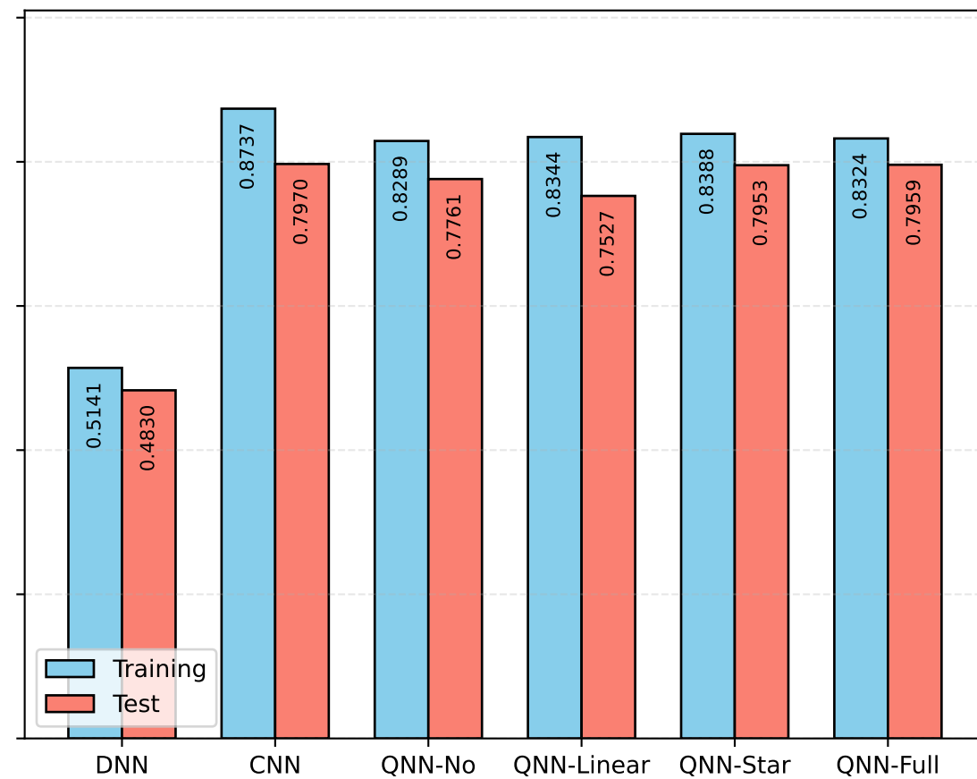
CIFAR-10
